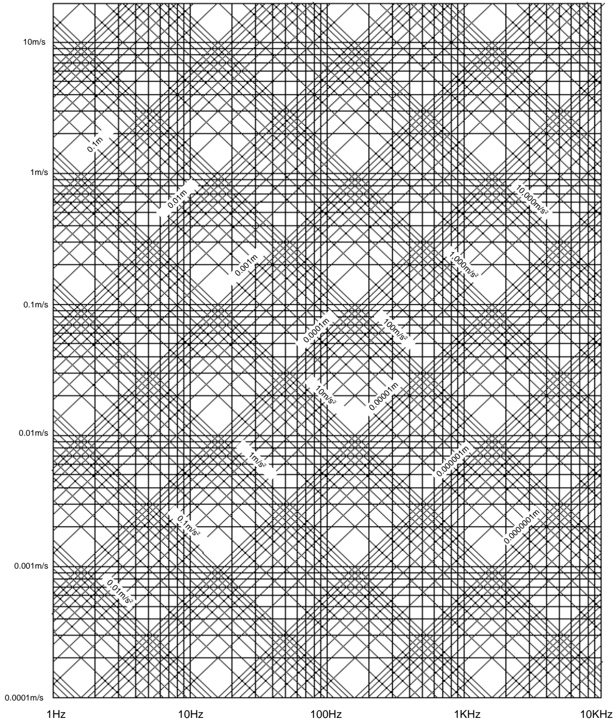
Velocity, Displacement and Acceleration - RMS or Peak
